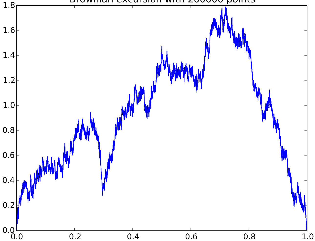
Brownian excursion with 200000 points
