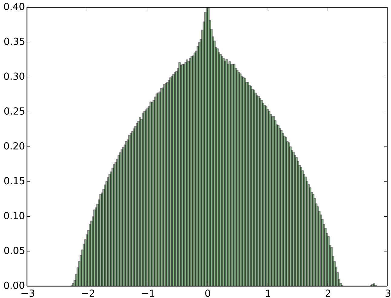
Spectrum of 50 Erdos Renyi random graphs ( n=5000 and average degree c=5 )
