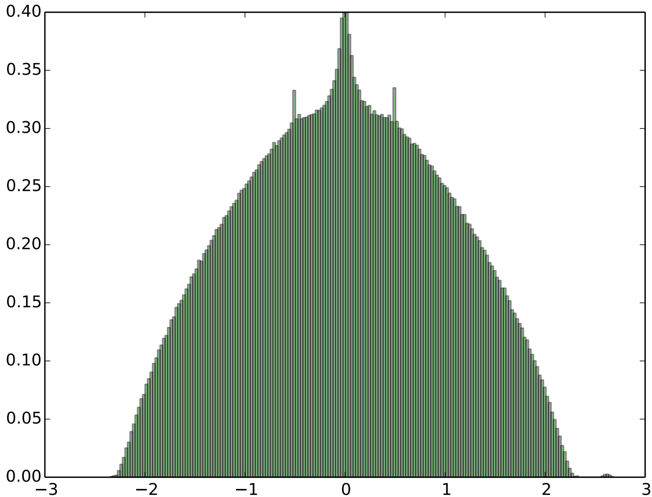
Spectrum of 50 Erdos Renyi random graphs ( n=5000 and average degree c=4 )
