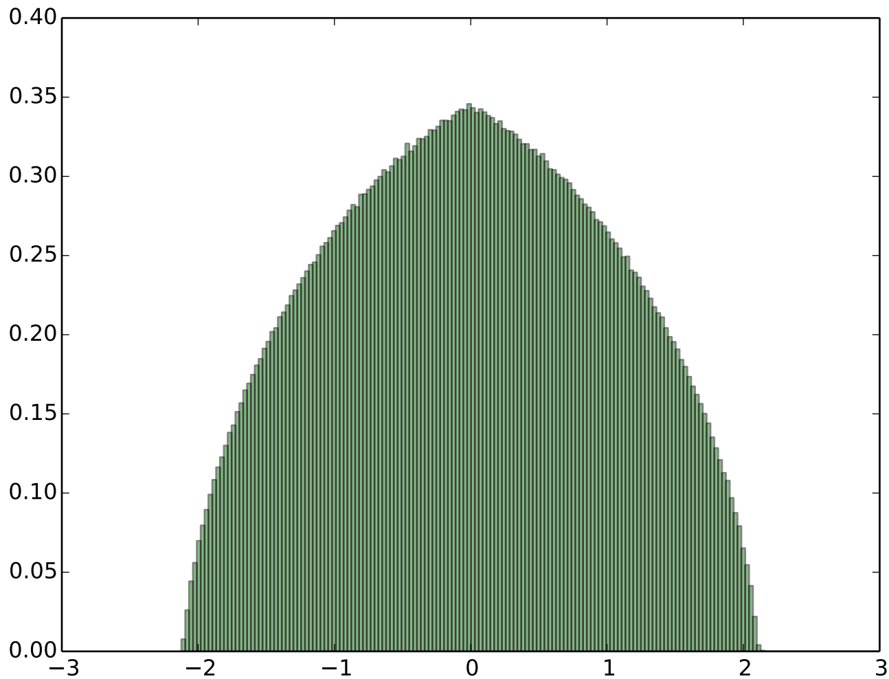
Spectrum of 50 Erdos Renyi random graphs ( n=5000 and average degree c=10 )
