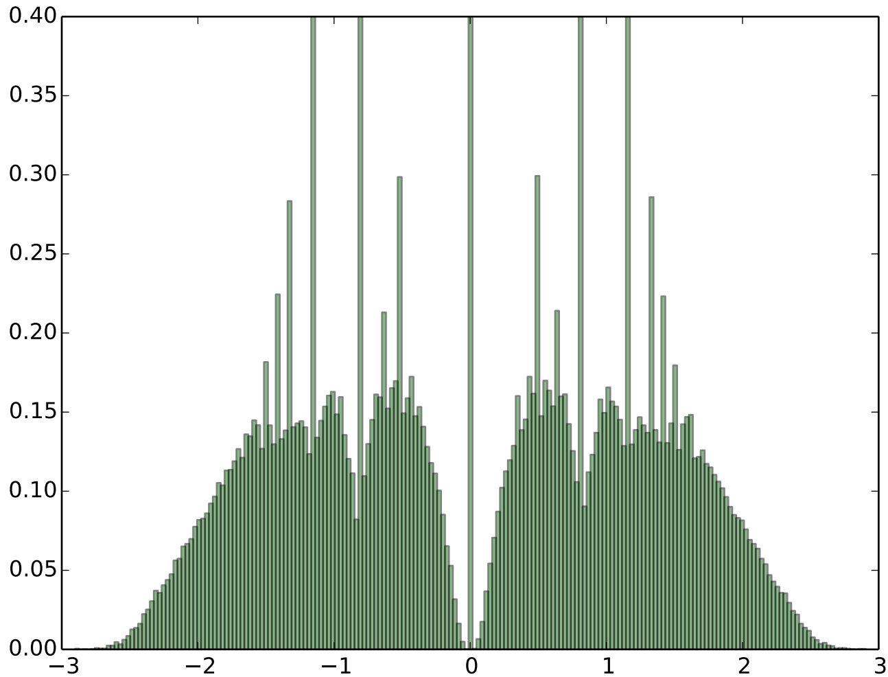
Spectrum of 50 Erdos Renyi random graphs ( n=5000 and average degree c=1.5 )
