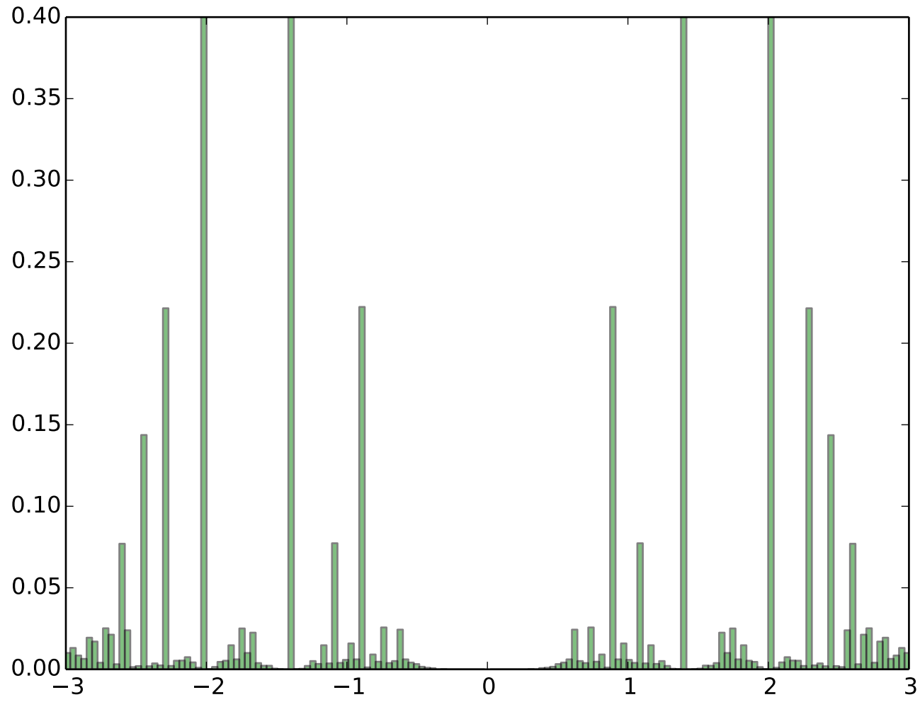
Spectrum of 50 Erdos Renyi random graphs ( n=5000 and average degree c=0.5 )
