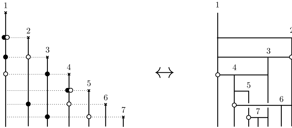
Figure 7: Graphical representation of the forward-time construction of RTCNs. On the left, the black and white dots represent the subexcedant sequences s^\bullet and s^\circ , respectively, and on the right the corresponding RTCN. At each step, the new lineage (marked by a cross) is linked to the black dot and the white dot. If these two dots fall on the same lineage, we get a branching.
