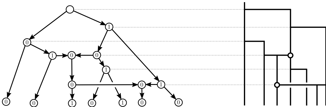
Figure 6: An example of a decorated RTCN (left) with its simplified representation (right). In the simplified representation, decorated lineages are indicated as follows: for branchings, they are drawn to the right; for reticulations, we add a white dot to indicate which parent of the reticulation points to a 1.
