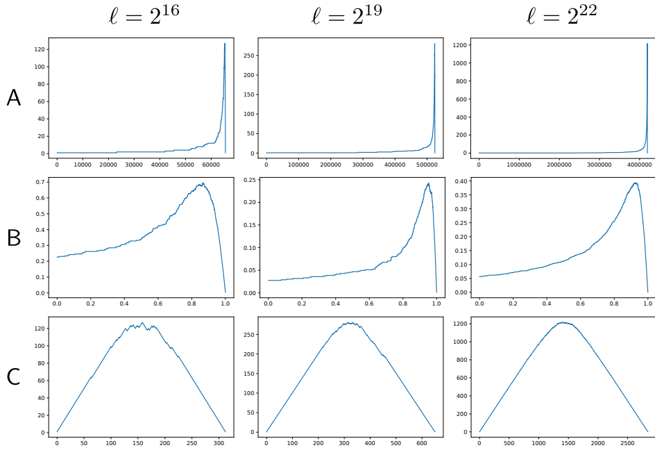
Figure 15: Individual trajectories of the processes described in the main text, for different values of \ell . A, the process X^{(\ell)} , B the process t \mapsto \frac{1}{\sqrt{\ell}} X^{(\ell)}_{\lfloor \ell - M\sqrt{\ell}(1-t) \rfloor} and C, the process \tilde{X}^{(\ell)} .
