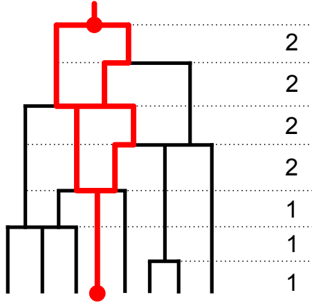
Figure 3: In red, the ancestry of a leaf and on the right the process counting the number of lineages in this ancestry.
