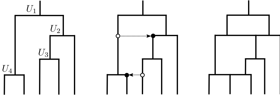
Figure 10: Example of the random construction of a RTCN from a ranked tree described in Proposition 3.5. Here, nothing happens for U_1 and U_3 . For U_2 and U_4 , the black dot represents the edge e and the white one the edge e' . Note that the modifications of branching events can be performed in any order, but that they have to be performed sequentially, so that contemporary edges remain well-defined at every step of the procedure.
