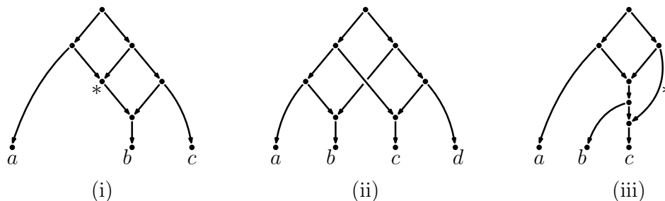
Figure 1: (i) A binary phylogenetic network that fails to be tree-child, since the only path from the vertex indicated by “*” to the leaves passes through a reticulation vertex; (ii) A tree-child network that cannot be ranked (i.e. does not correspond to any RTCN); (iii) A tree-child network that is not a normal network, as the arc indicated by “*” is redundant (see Definition 1.7).
