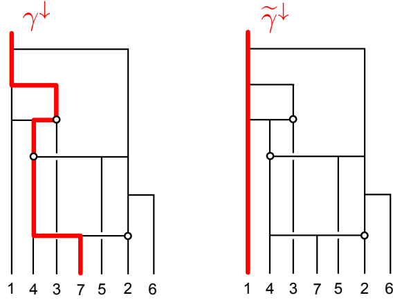
Figure 12: On the left, the path \gamma^\downarrow and on the right the path \tilde{\gamma}^\downarrow corresponding to the lineage of the first particle.
