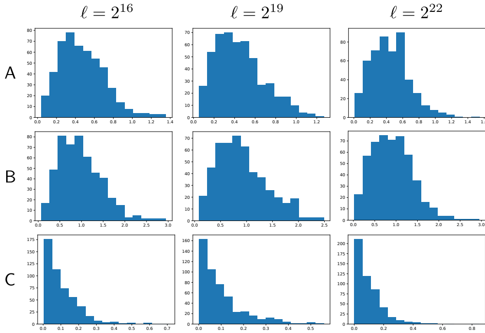
Figure 16: Distribution of some statistics of X^{(\ell)} for M = 10 and 500 trajectories. A, \frac{1}{\sqrt{\ell}} \max\{X_k^{(\ell)} : 0 \leq k \leq \ell - 2\} ; B, \frac{1}{\sqrt{\ell}} (\ell - \arg\max\{X_k^{(\ell)} : 0 \leq k \leq \ell - 2\}) and C, \frac{1}{\sqrt{\ell}} X^{(\ell)}_{\lfloor \ell - M\sqrt{\ell} \rfloor}
