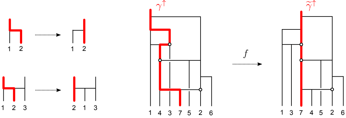
Figure 13: Illustration of the deterministic procedure used to “straighten” the path \gamma^\uparrow in order to make it coincide with the lineage of the first particle. Left: the local modifications that are made each time a branching or a reticulation is encountered; these essentially consist of swapping lineages. Right: an example of application of the procedure to a RTCN.
