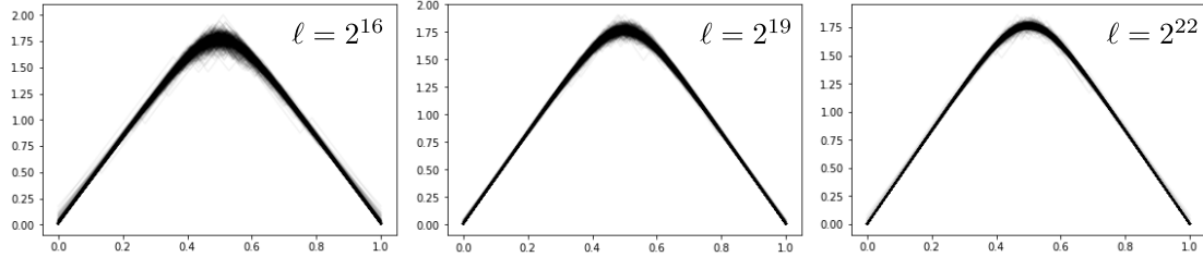
Figure 4: 500 superimposed trajectories of the process \tilde{X}^{(\ell)} , rescaled so that their domain is [0, 1] and that the total area under each curve is equal to 1.
