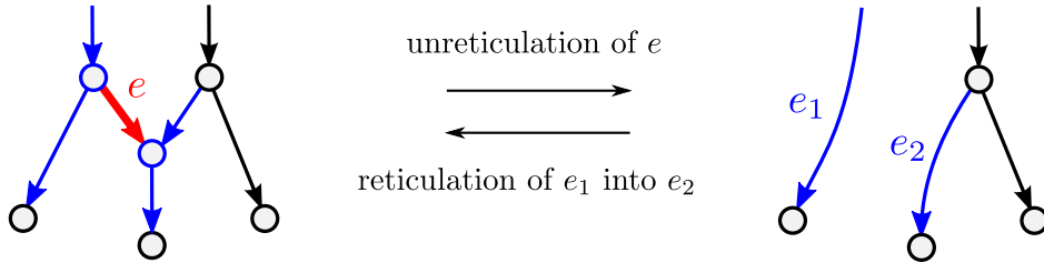
Figure 8: The operations of unreticulation and reticulation.
