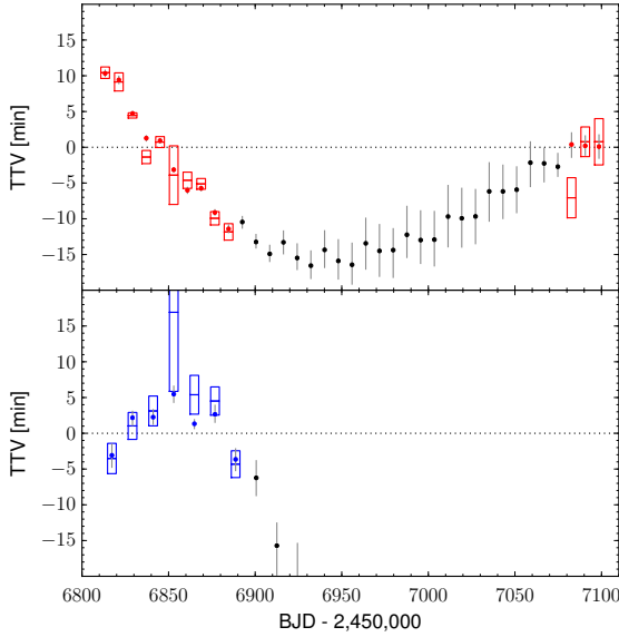
Figure 4. Comparison of the TTVs derived by the photo-dynamic model (as circles) with TTVs derived using a standard transit fitting (as boxes with the size of the 1 sigma error) for planet b (top panel) and planet c (bottom panel). For each planet we use the respective ephemeris derived using the photo-dynamic estimated values of only the observed transits which are marked in red for planet b and in blue for planet c.
