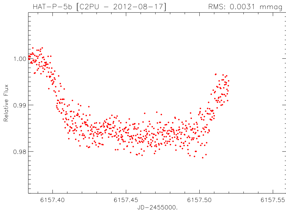
Figure 3. The light curve of the transiting exoplanet HAT-P-5b, with C2PU W-Tel (August 17 th , 2012).
