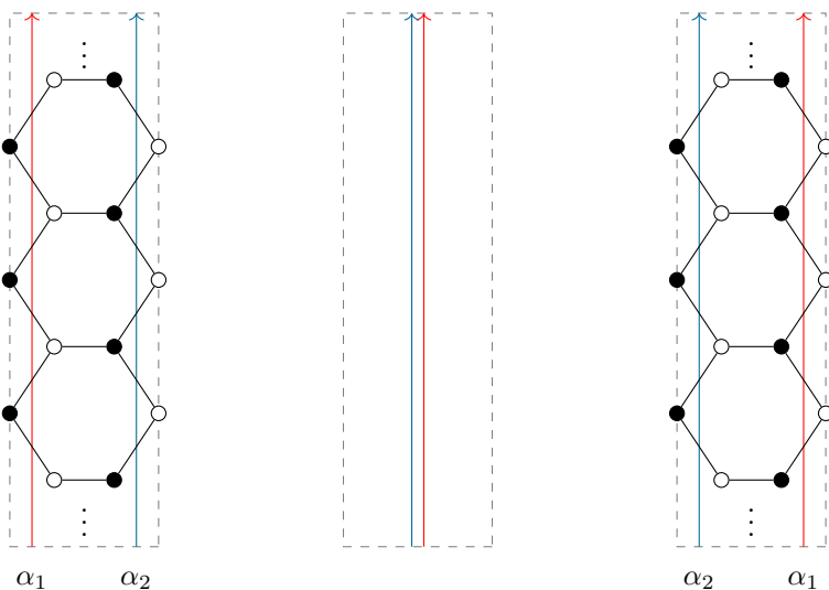
Figure 3: The geometric R -matrix transformation and the homotopy of zig-zag paths. The red and blue zig-zag paths on either side of the cyclic chain of hexagons interchange positions, while all other zig-zag paths are left unchanged.
