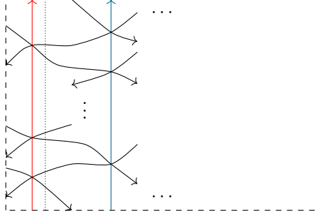
Figure 11: The blue strand runs parallel to the left side of R' , i.e. there are no triple points strictly between the red strand and the blue strand.
