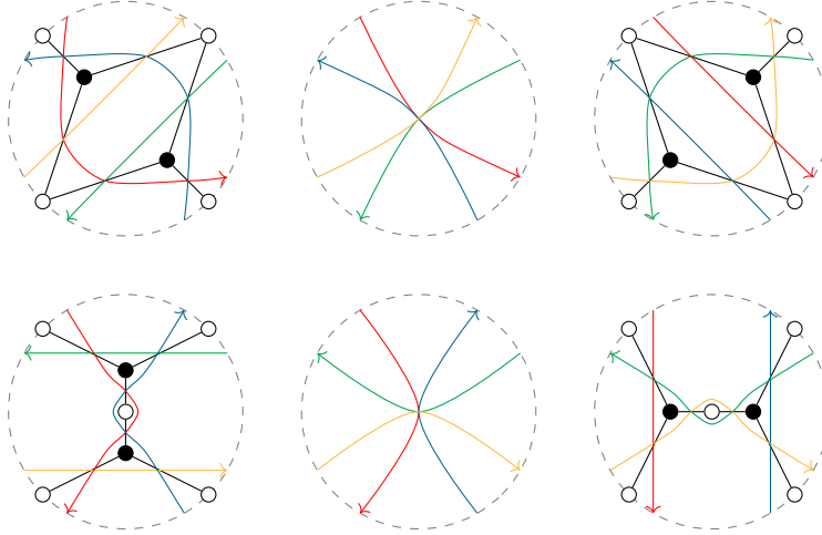
Figure 1: The elementary transformations: the spider move (above) and the resplit move (below), along with the corresponding homotopies of zig-zag paths.
