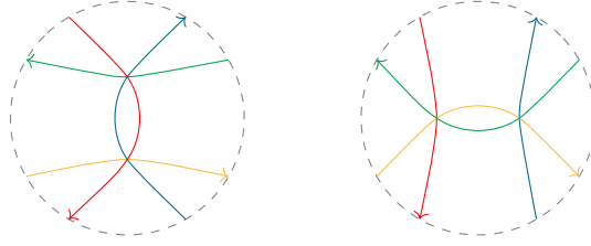
Figure 7: The 2 – 2 move.
