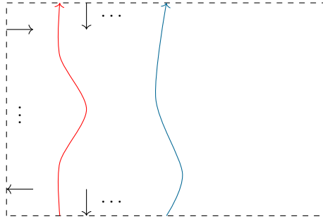
Figure 8: The configuration at the end of Step 1. The red strand is \alpha_1 and the blue strand is \alpha_2 . There are no other end-points of strands between the end-points of \alpha_1 and the black strands.
