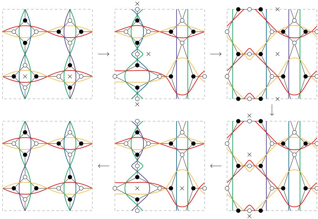
Figure 4: A generalized cluster transformation for the square-octagon graph, along with the homotopy of zig-zag paths. The faces/white-vertices/chain of hexagons at which we are doing transformations are marked by \times 's. We have colored the two blue zig-zag paths with different shades of blue to distinguish them. The result of the homotopy is that the two blue zig-zag paths are swapped, while all other zig-zag paths return to their initial positions.
