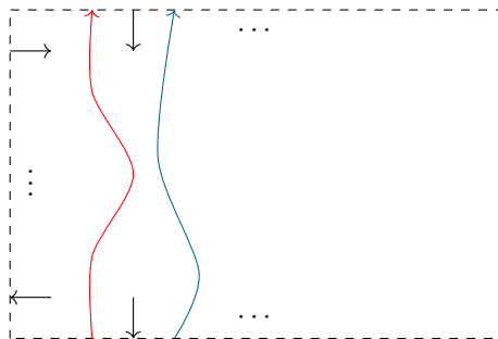
Figure 9: There are no other end-points of strands between the end-points of \alpha_1 and the black strands (resp. between the end-points of \alpha_2 and the black strands).
