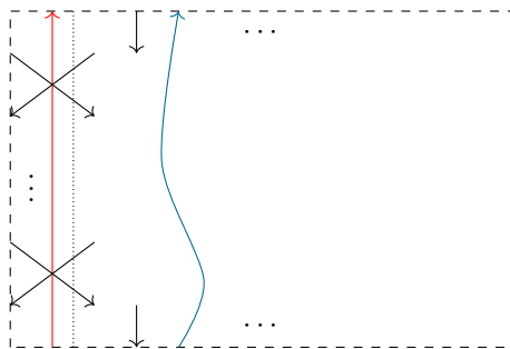
Figure 10: The red strand runs parallel to the left side of R , i.e. there are no triple points strictly between the red strand and the left side of R .
