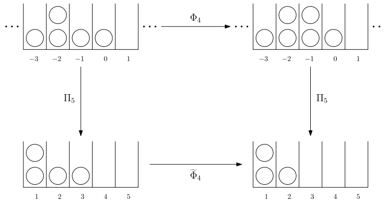
Fig. 3. “Commutation” of \Pi_5 with \Phi_4 and \tilde{\Phi}_4 .
