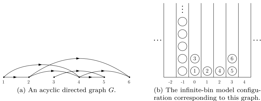
Fig. 4. From a Barak–Erdős graph to an infinite-bin model configuration.
