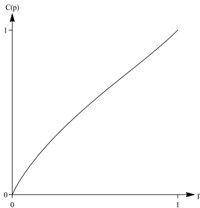
Fig. 1. Plot of an approximation of C(p) , using 600,000 iterations of an infinite-bin model, for values of p that are integer multiples of 0.02.
