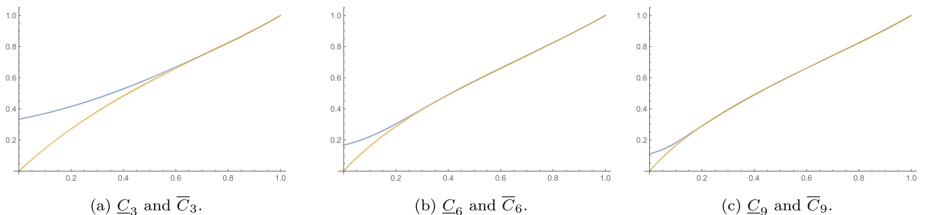
Fig. 5. Lower and upper bounds \underline{C}_k and \overline{C}_k for C , for k \in \{3, 6, 9\} .
