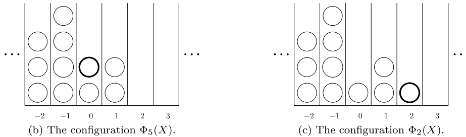
Fig. 2. Action of two moves on a configuration.
