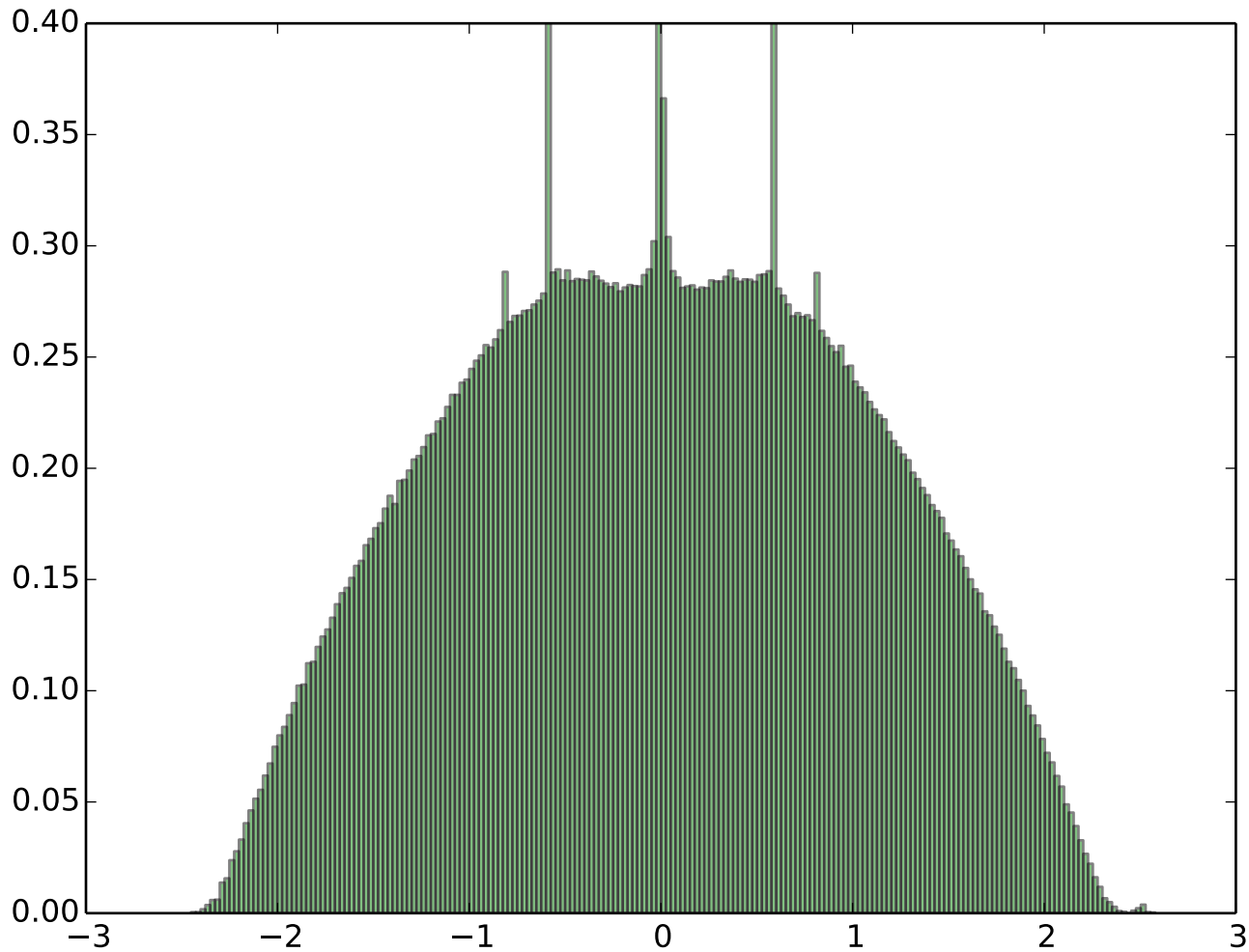
Spectrum of 50 Erdos Renyi random graphs ( n=5000 and average degree c=3 )
