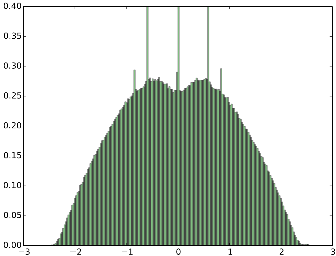
Spectrum of 50 Erdos Renyi random graphs ( n=5000 and average degree c=2.8 )
