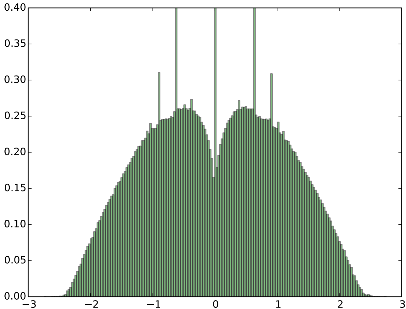
Spectrum of 50 Erdos Renyi random graphs ( n=5000 and average degree c=2.5 )
