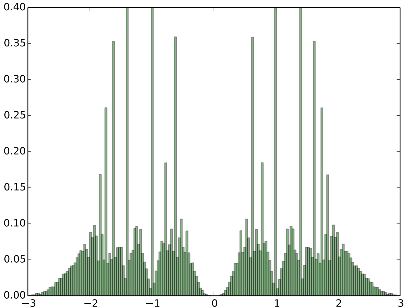
Spectrum of 50 Erdos Renyi random graphs ( n=5000 and average degree c=1 )
