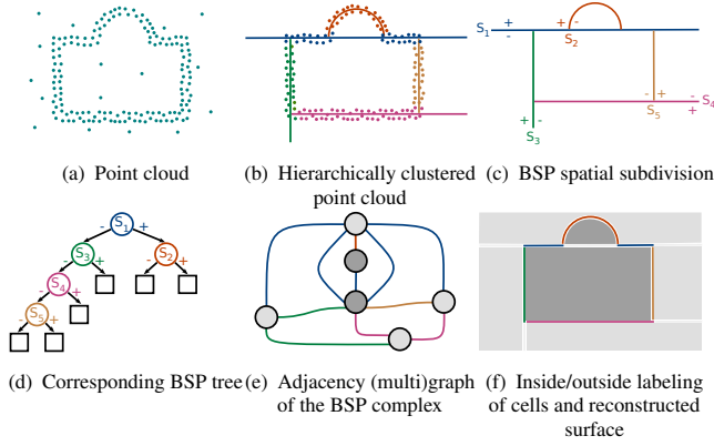
Figure 1: Generalized BSP trees for hierarchical clustering of point clouds and boundary representation of piecewise-primitive surfaces.
