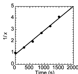
Fig. 4. Kinetics of the reaction of morpholine (2 mM) with the cationic complex [(\eta^3\text{-CH}_2\text{-CH-CH}_2)\text{Pd}(\text{PAr}_3)_2]^+\text{BF}_4^- ( \text{Ar} = 4\text{-Me-C}_6\text{H}_4 ) ( \mathbf{2b}^+ , \text{BF}_4^- ) ( C_0 = 1 mM) in DMF at 25^\circ\text{C} , monitored by UV spectroscopy at 296 nm. Variation of 1/x versus time ( x = ([\mathbf{8}]_{\text{lim}} - [\mathbf{8}])/[\mathbf{8}]_{\text{lim}} = (D_{\text{lim}} - D)/D_{\text{lim}} with D : absorbance of \mathbf{8} at t and D_{\text{lim}} : final absorbance of \mathbf{8} . 1/x = 2k_{\eta 3}C_0t + 1 [25].
