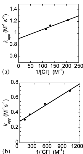
Fig. 5. Kinetics of the reaction of morpholine with the cationic complexes [(\eta^3\text{-CH}_2\text{-CH-CH}_2)\text{Pd}(\text{PAR}_3)_2]^+ \text{BF}_4^- in DMF in the presence of various amount of \text{Cl}^- ions added as n\text{Bu}_4\text{NCl} at 25^\circ\text{C} , monitored by UV spectroscopy. Variation of k_{\text{app}} versus the reciprocal of \text{Cl}^- concentration (see Eq. (11)). (a) \text{Ar} = 4\text{-Cl-C}_6\text{H}_4 ( 2\text{a}^+ , \text{BF}_4^- , C_0 = 0.5 \text{ mM} ), morpholine (15 equivalent); (b) \text{Ar} = 4\text{-Me-C}_6\text{H}_4 ( 2\text{b}^+ , \text{BF}_4^- , C_0 = 1 \text{ mM} ), morpholine (2 equivalent).
