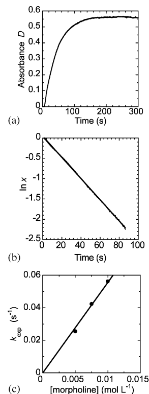
Fig. 3. Kinetics of the reaction of morpholine with the cationic complex [(\eta^3-CH_2-CH-CH_2)Pd(PAr_3)_2]^+ BF_4^- ( Ar = 4-Cl-C_6H_4 ) ( 2a^+ , BF_4^- ) (0.5 mM) in DMF containing nBu_4NBF_4 (0.3 M) at –25 °C, monitored by UV spectroscopy. (a) Absorbance at 323 nm of the Pd^0 complex 8 versus time, after addition of 10 equivalent morpholine; (b) variation of \ln x versus time ( x = ([8]_{lim} - [8])/[8]_{lim} = (D_{lim} - D)/D_{lim} with D : absorbance of 8 at t and D_{lim} : final absorbance of 8 determined in Fig. 1a). \ln x = -k_{exp}t ; (c) reaction order in morpholine: plot of k_{exp} versus the morpholine concentration. k_{exp} = k_{\eta^3}[morpholine] .
