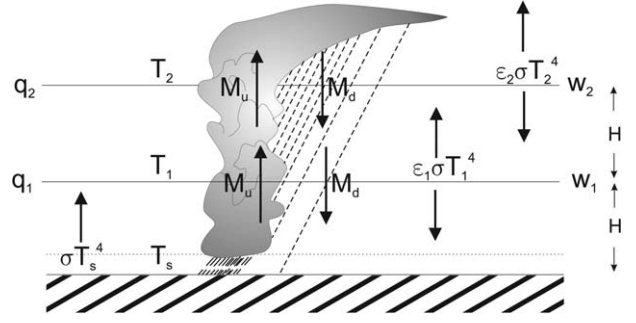
Figure 1. The two-layer model. Surface temperature and the temperatures of each layer are specified and constant. The emissivities, \varepsilon , updraft and downdraft mass fluxes, M_u and M_d , large-scale vertical velocities, w , and specific humidities, q , are variable. The vertical arrows depict the convective and radiative fluxes.
