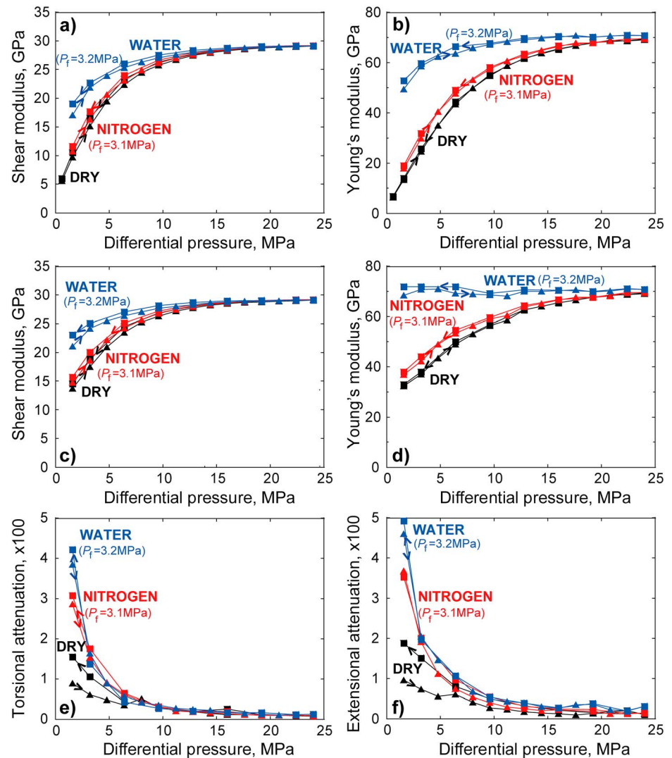
Figure 13. Results of resonant bar experiments on the cracked glass rod specimen FDL2, conducted at resonance frequencies of 1.1–1.5 kHz (torsional mode) and 1.5–2.4 kHz (extensional mode), under dry, nitrogen-saturated, and water-saturated conditions in sequence. (a) Shear modulus, (b) Young's modulus, (c) shear modulus adjusted for interfacial compliance as explained in the text, (d) Young's modulus adjusted for interfacial compliance as explained in the text, (e) torsional, and (f) extensional mode attenuation uncorrected for any interfacial contribution. The uncertainty of modulus is \pm 1\% . Arrows along curves indicate pressure path during the experiment.
