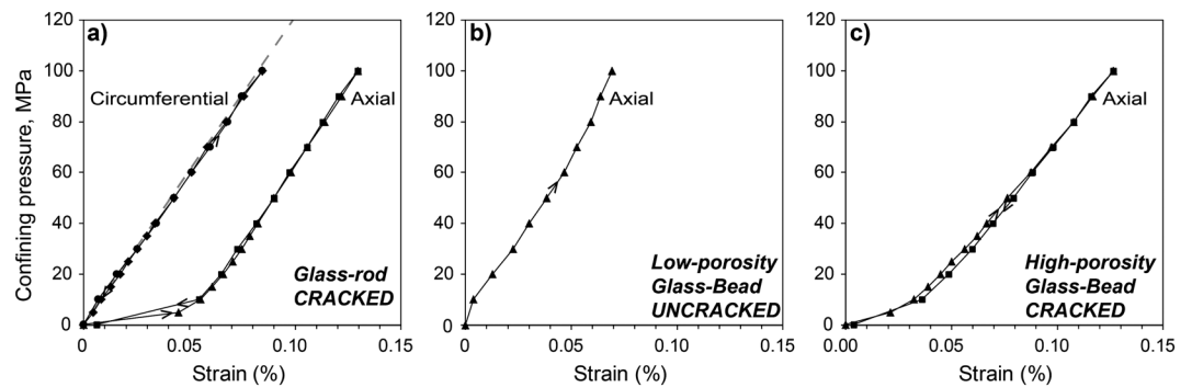
Figure 9. (a) The pressure dependence of the axial and circumferential strains for a cracked glass rod specimen, compared with the elastic strain expected for a bulk modulus of 40 GPa (dashed grey line); (b) the axial strain for an uncracked low-porosity glass bead specimen; and (c) the axial strain for a cracked high-porosity glass bead specimen. Arrows along curves indicate pressure path during the experiment.
