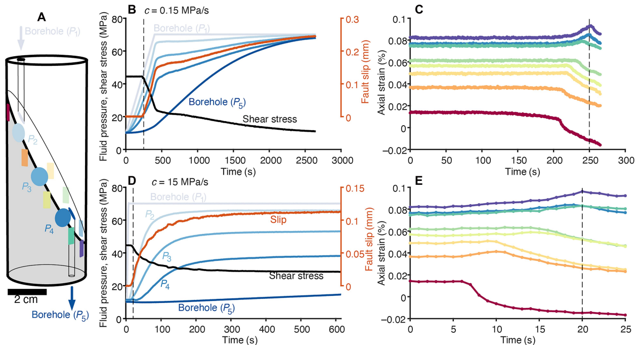
Fig. 1. Experimental methods. (A) Schematic representation of the sample assembly used in this study. The host rock is Westerly Granite. Rectangles indicate the location of strain gauges around the fault. The injection borehole and the measurement borehole correspond to pressures P_1 and P_5 , respectively. (B) Evolution of macroscopic shear stress, macroscopic fault slip, and fluid pressure measured at five different locations [colors correspond to those shown in (A)] during an injection performed at \tau_0/\tau_p = 0.6 , with a constant pressure rate of c = 0.15 MPa/s. (C) Evolution of axial strain recorded by the strain gauge array before the onset of macroscopic slip, indicated by the dashed line. The strain data are organized by distance from the injection site. Colors match those of the markers shown in (A). (D) Same as (B), but for the injection conducted at \tau_0/\tau_p = 0.6 with a constant pressure rate of c = 15 MPa/s. (E) Same as (C), but for the injection conducted at \tau_0/\tau_p = 0.6 with a constant pressure rate of c = 15 MPa/s.
