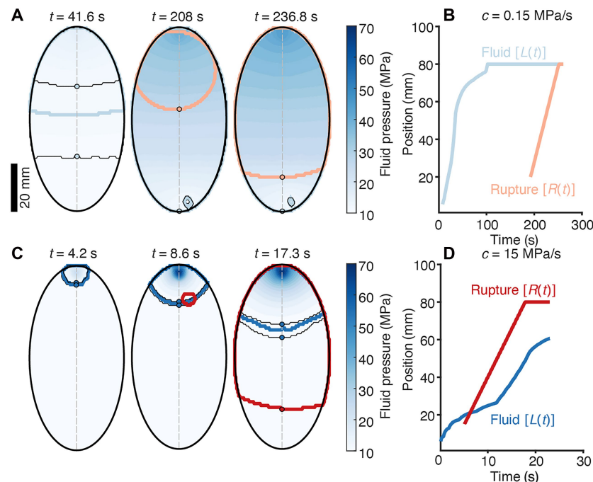
Fig. 2. Inversion of R and L during fluid injection. (A) Snapshots at three different times illustrating the propagation of the fluid pressure front L (blue) and the slip front R (reddish line) during an injection performed at \tau_0/\tau_p = 0.6 with a constant pressure rate c = 0.15 MPa/s. The color scale represents fluid pressure (same as in Fig. 3). Thin black contours indicate the position of the fluid pressure front L for thresholds of 10.7 and 11.3 MPa, while the thick blue contour corresponds to 11 MPa. Colored markers show the positions of the slip front R (reddish colors) and the pressure front L (bluish colors) along the fault trace (dashed line). (B) Temporal evolution of the front positions R(t) and L(t) along the fault for the same injection conditions ( \tau_0/\tau_p = 0.6 , c = 0.15 MPa/s). (C) Same as (A), but for an injection with a higher constant pressure rate c = 15 MPa/s. (D) Same as (B), but for c = 15 MPa/s.
