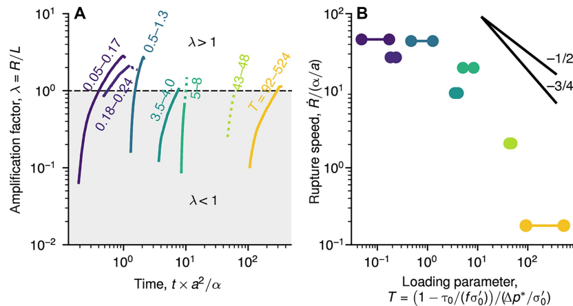
Fig. 4. Influence of the loading parameter T on slip and fluid propagation. (A) Ratio \lambda = R(t)/L(t) as a function of scaled time for all injections. The colored solid lines show the evolution of \lambda during the period when both the slip front R(t) and the fluid pressure front L(t) are propagating along the fault. The colored dashed lines represent that the evolution of \lambda after either the fluid pressure front L(t) or the slip front R(t) has reached the bottom edge of the fault. The black dashed line corresponds to \lambda = 1 and marks the transition between the regime in which the slip front lags behind the fluid pressure front ( \lambda < 1 , gray area) and the regime in which the slip front outpaces the fluid pressure front ( \lambda > 1 ). (B) Scaled rupture speed as a function of the loading parameter T .
