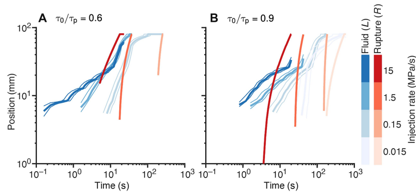
Fig. 3. One-dimensional propagation of rupture R(t) and fluid pressure L(t) . (A) Evolution of the rupture dimension (reddish colors) and fluid front position (bluish colors) along the fault length (Fig. 2) as a function of time for injections conducted at \tau_0/\tau_p = 0.6 . L(t) represents the location of the fluid front for a threshold of 1 MPa above the initial, uniform pressure field (solid lines), \pm 0.3 MPa (thin lines). The reddish and bluish color scales correspond to the values of pressurization rate c used in each injection. (B) Same as (A), but for injections conducted at \tau_0/\tau_p = 0.9 .
