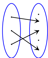
f injective
